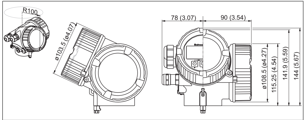
10 Housing GT18 (316L); Dimensions in mm (in)
