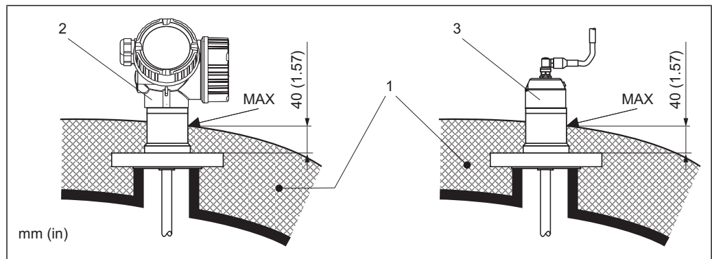
7 Process connection with flange - FMP51, FMP52
