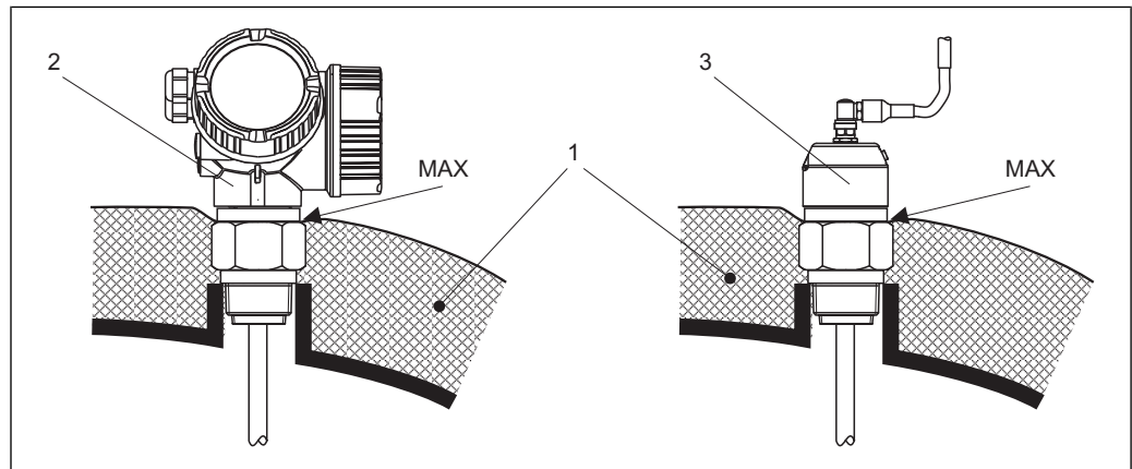
6 Process connection with thread - FMP51
