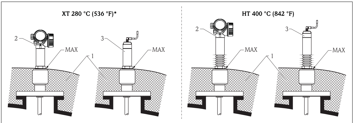
9 Process connection with flange – FMP54, sensor version XT and HT
