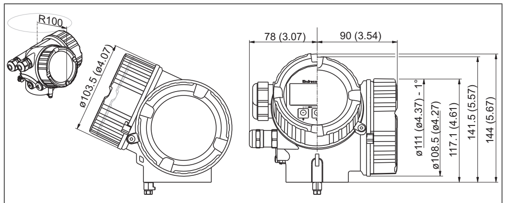
12 Housing GT20 (Alu coated); Dimensions in mm (in)
