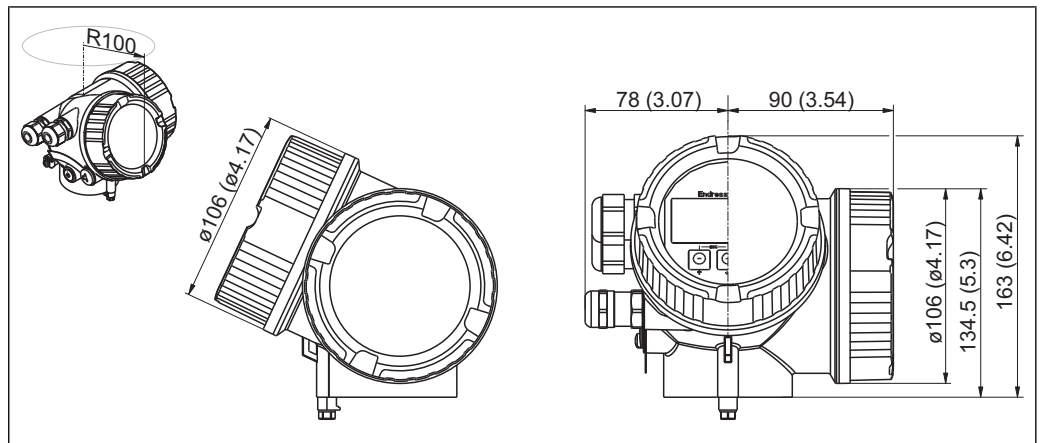
11 Housing GT19 (Plastics PBT); Dimensions in mm (in)
