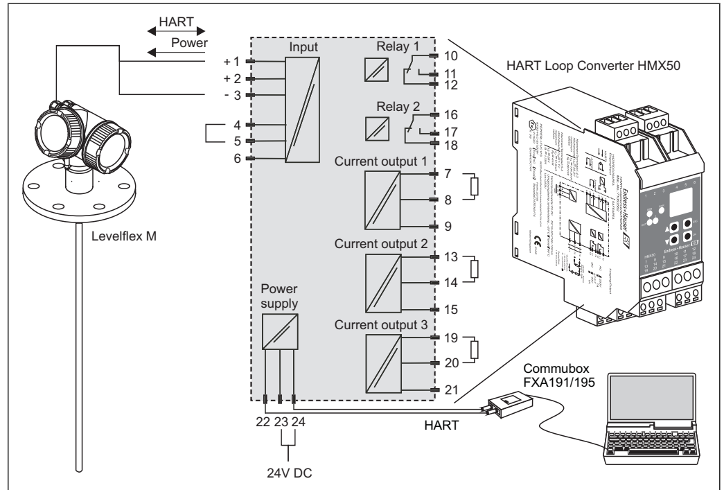
4 Connection diagram for HART loop converter HMX50 (example: passive 2-wire device and current outputs connected as power source)
