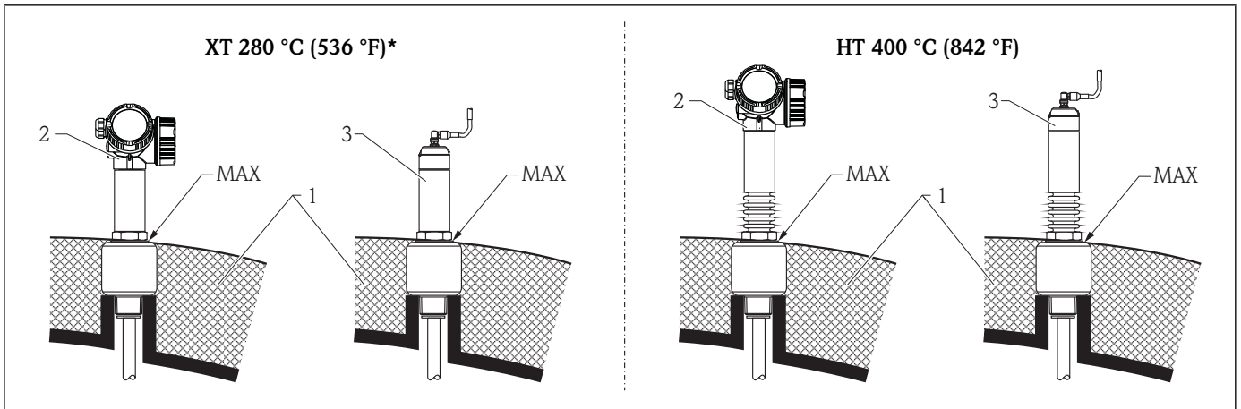
8 Process connection with thread – FMP54, sensor version XT and HT
