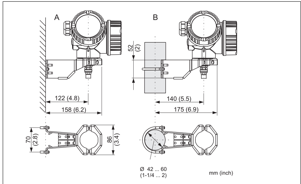
13 Mounting bracket for the electronics housing
