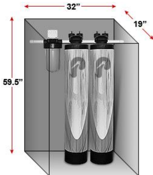
SYSTEM DIMENSIONS - PSE2000
