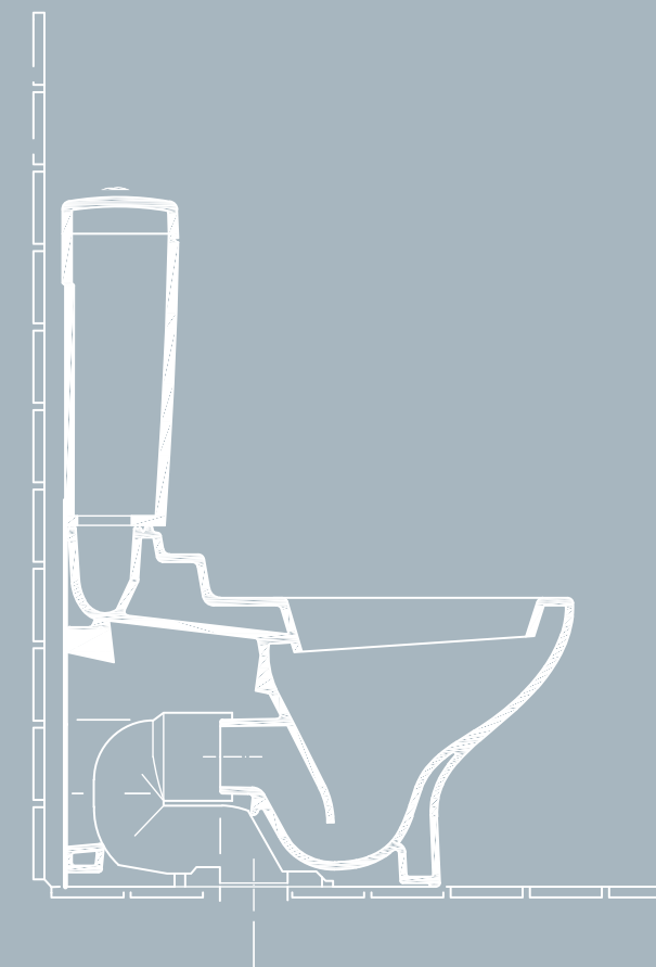
Install with Villeroy & Boch's Vario Drainbend for floor waste outlets.
